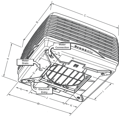
CABINET DETAILS
